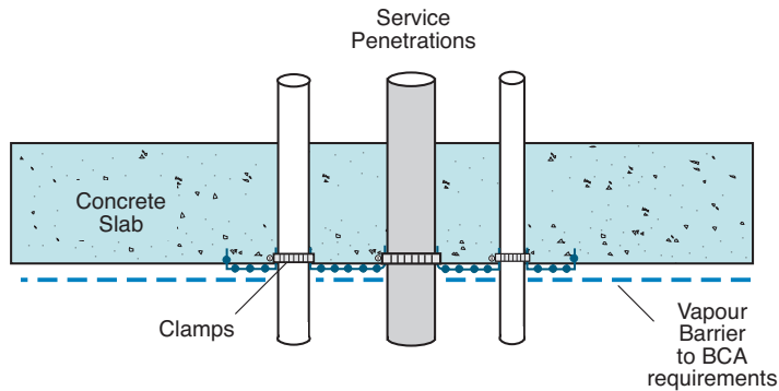
Installation at Base of Slab – pre-pour
