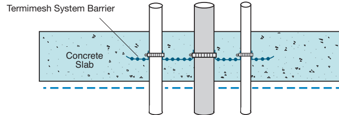
Installation in Centre of Slab – pre-pour
