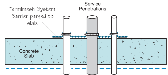
Installation on Top of Slab – post-pour
